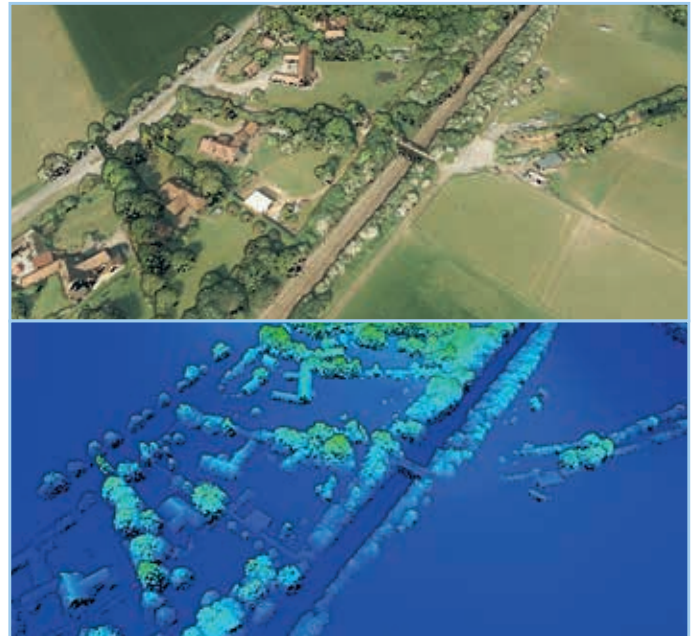
Figure 14 - Rail corridor
